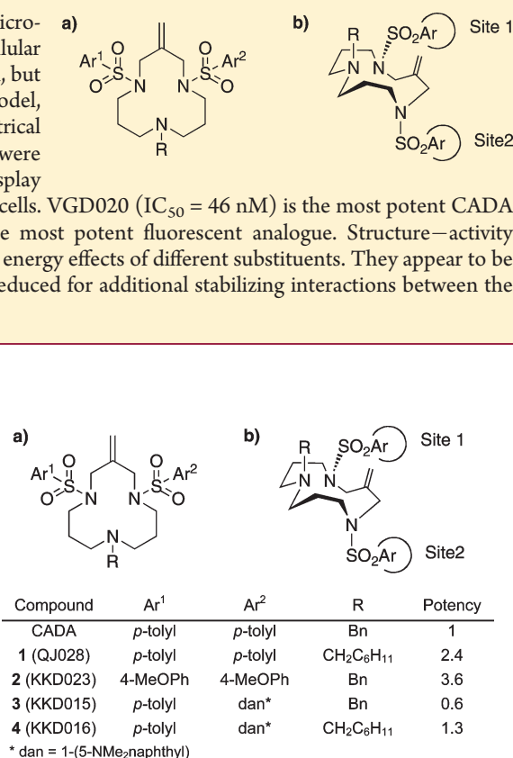
Figure 1. (a) Structures of previously synthesized CADA compounds, including unsymmetrical analogues 3 and 4. (b) Proposed unsymmetrical two-site binding model. Potency = IC_{50}(\text{CADA})/IC_{50}(\text{compound}) . IC_{50} is for CD4 down-modulation in MT-4 cells (ref 30).
