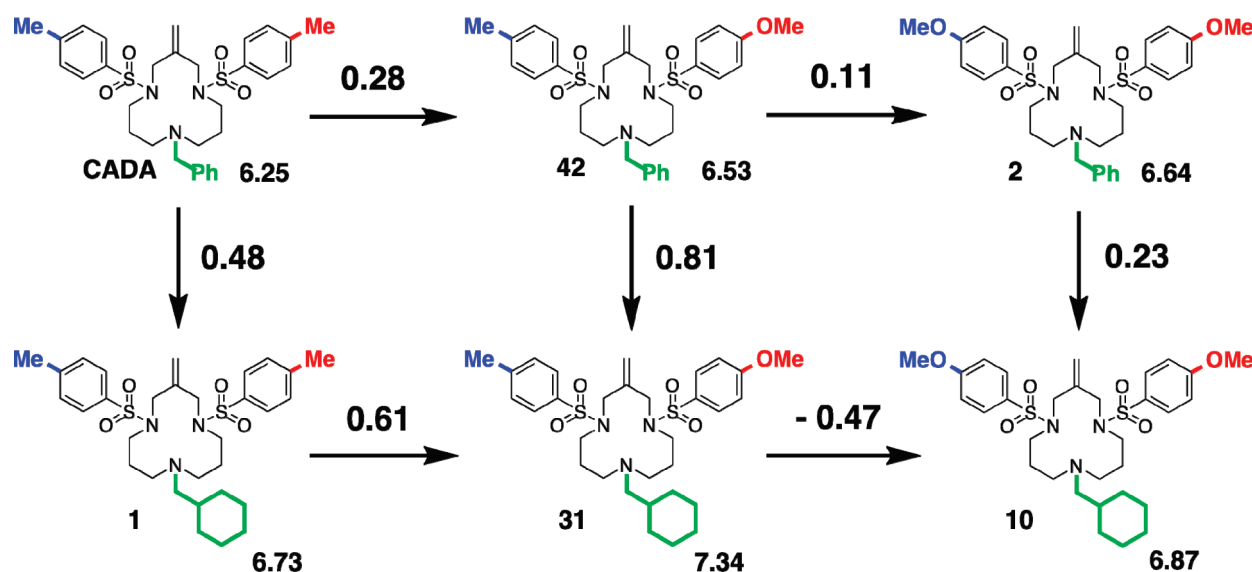
Figure 2. Thermodynamic cycle comparing energy effects of substitutions, starting with CADA (upper left). The pIC_{50} for CD4 down-modulation is given at lower right of each compound structure. Numbers above or beside each arrow represent change in pIC_{50} for each substitution.
