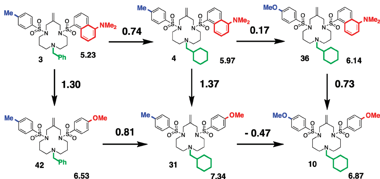
Figure 3. Thermodynamic cycle comparing energy effects of substitutions, starting with 3 (upper left). The pIC 50 for CD4 down-modulation is given at lower right of each compound structure. Numbers above or beside each arrow represent change in pIC 50 for each substitution.
